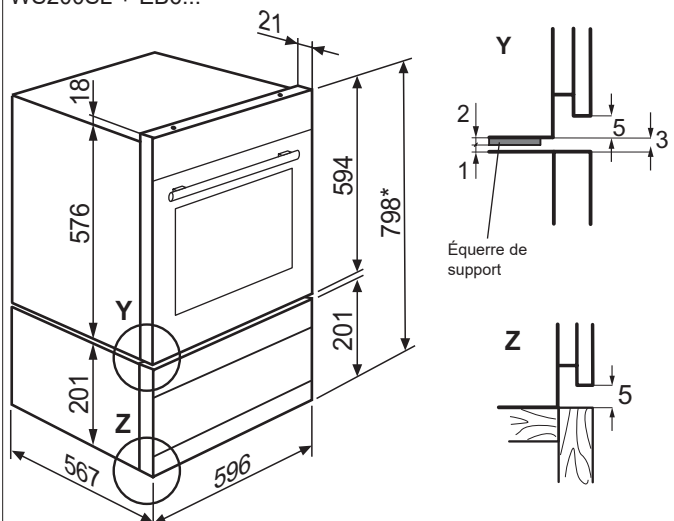
Tiroir chauffant + four encastrable WS200SL + EB6...
