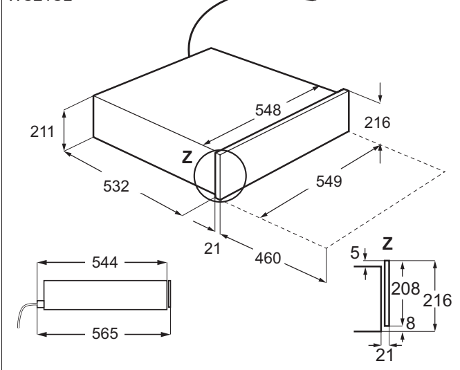
Tiroir chauffant WS21SL
