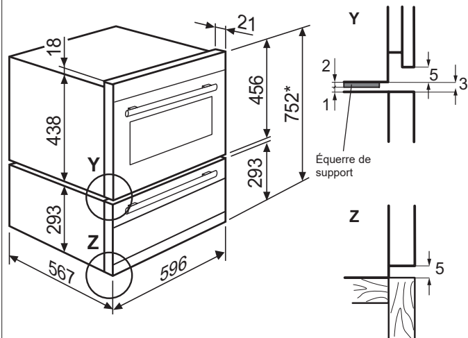
Tiroir chauffant + four encastrable Compact 45 WS290SL... + EB4...
