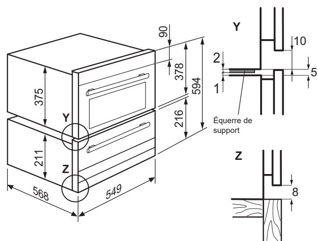
Tiroir chauffant + four encastrable Compact 38 WS21SL + EB3...
