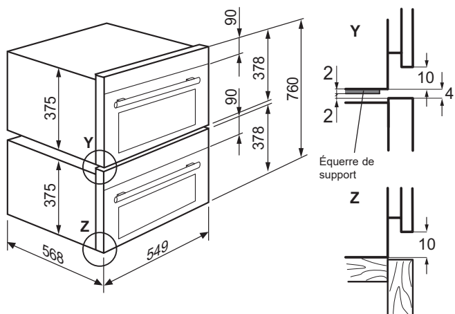
Four encastrable Compact 38 + four encastrable Compact 38 EB3... + EB3... (SMS 6/6)
