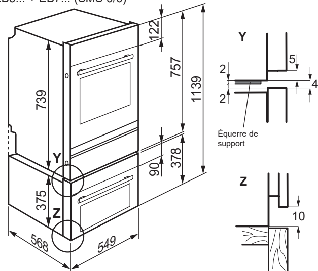
Four encastrable Compact 38 + four encastrable EB3... + EB7... (SMS 9/6)
