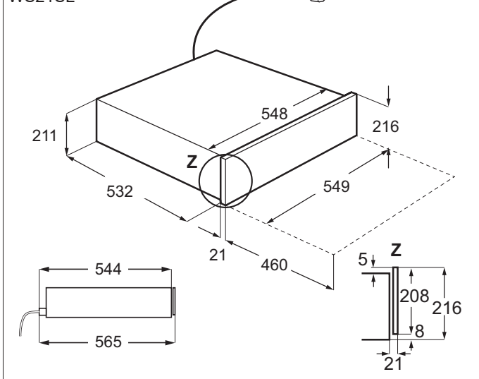
Cassetto scaldavivande WS21SL
