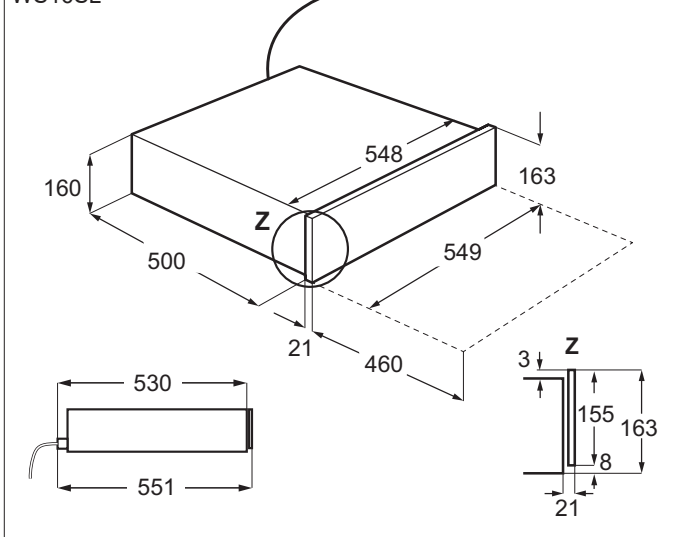
Cassetto scaldavivande WS16SL
